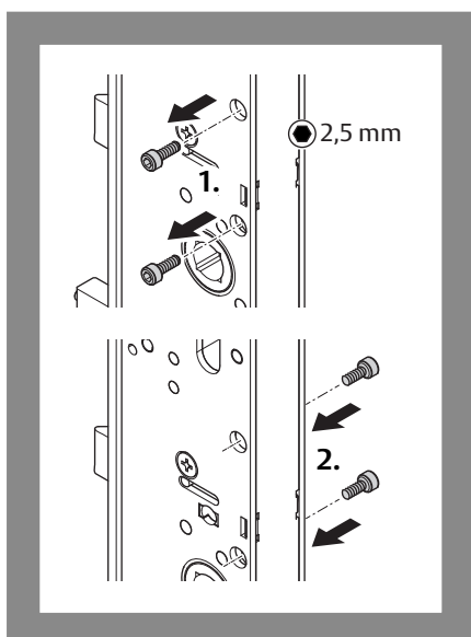
Fig. 12: Adjust the panic side
