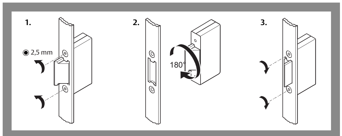
Fig. 10: Adjust the closing direction of the latch lock 807-10 to the control latch
