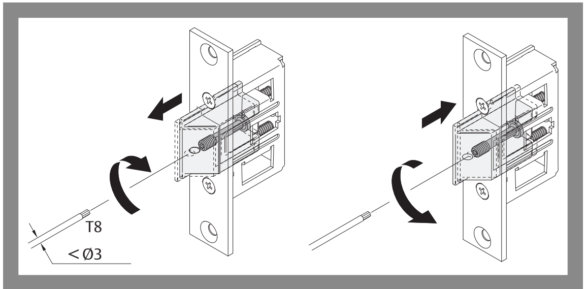
Fig. 11: Adjusting the latch range of latch lock 807-10
