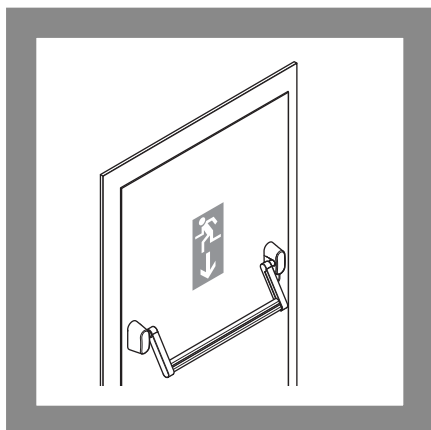
Fig. 16: A panic door according to DIN EN 1125,
